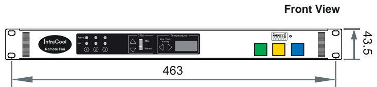
Front View
