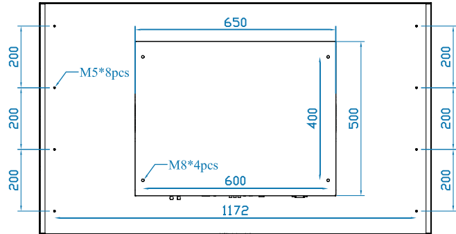
Rear View
