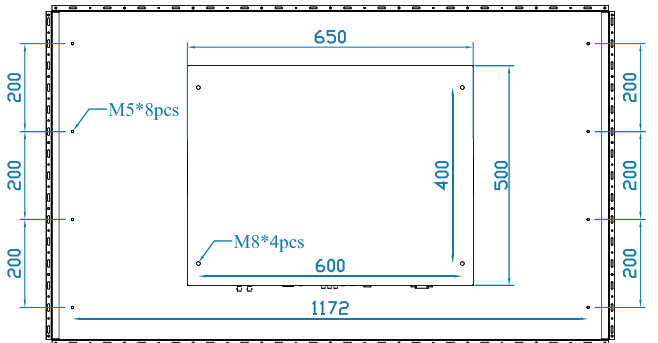
Rear View
