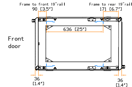
19" rail position
