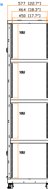
19" rail position
