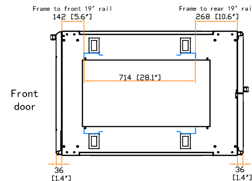
19" rail position
