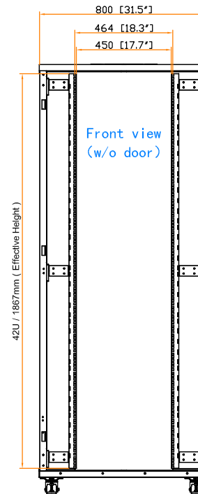
19" rail position
