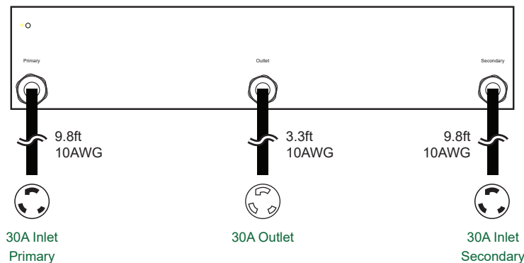
Circuit Details : 30A NEMA L6-30R connector
